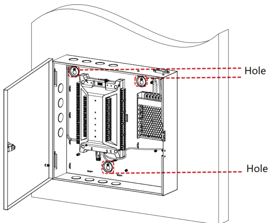
Figure 3-2 Hang Chassis
