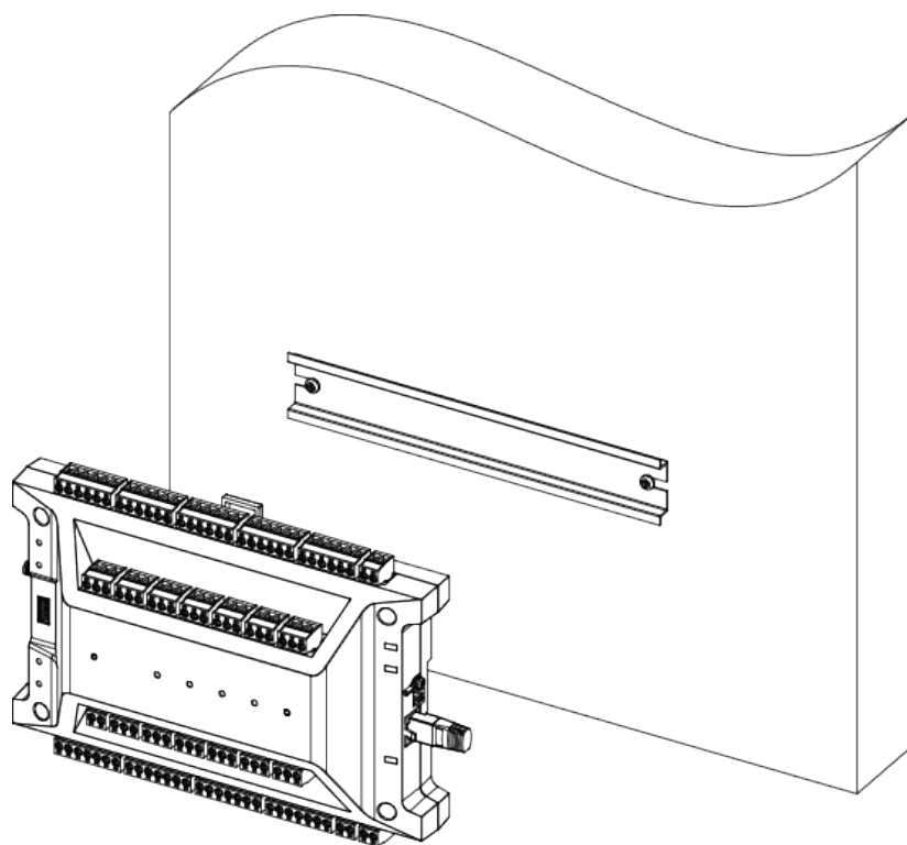
Figure 3-5 Fix Device
