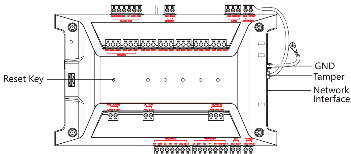
Figure 1-2 Appearance and Interfaces of 1-Door Access Controller Main Board
