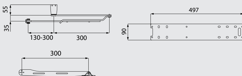
Fixing plate
