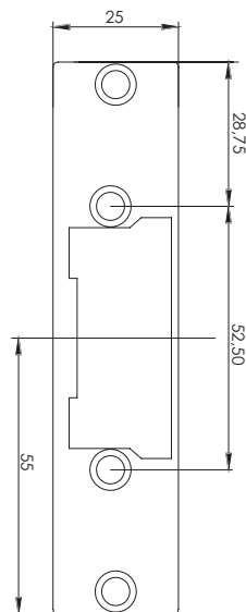
YB (20)
