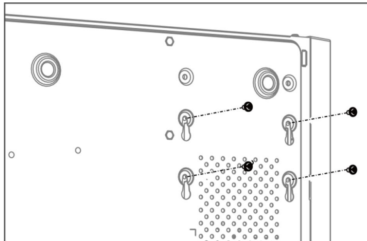
Figure 1-10 Fix HDD to Device Bottom
