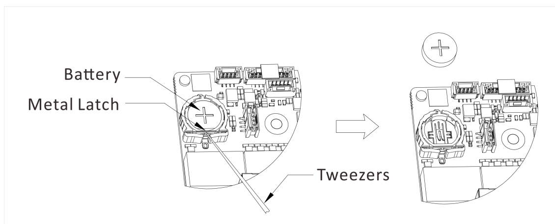
Figure 1-11 Remove Battery
