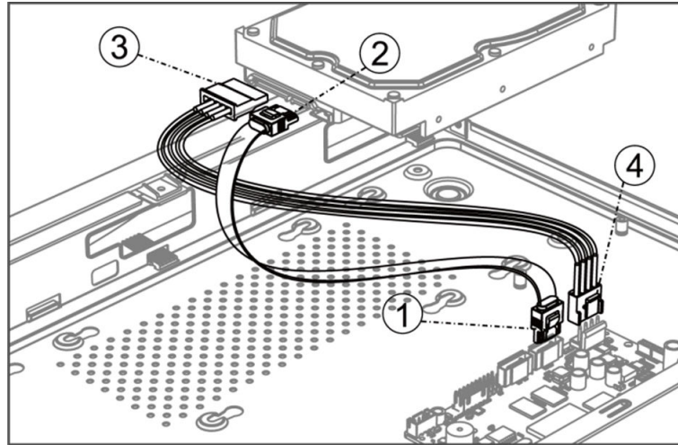
Figure 1-9 Connect Cables
