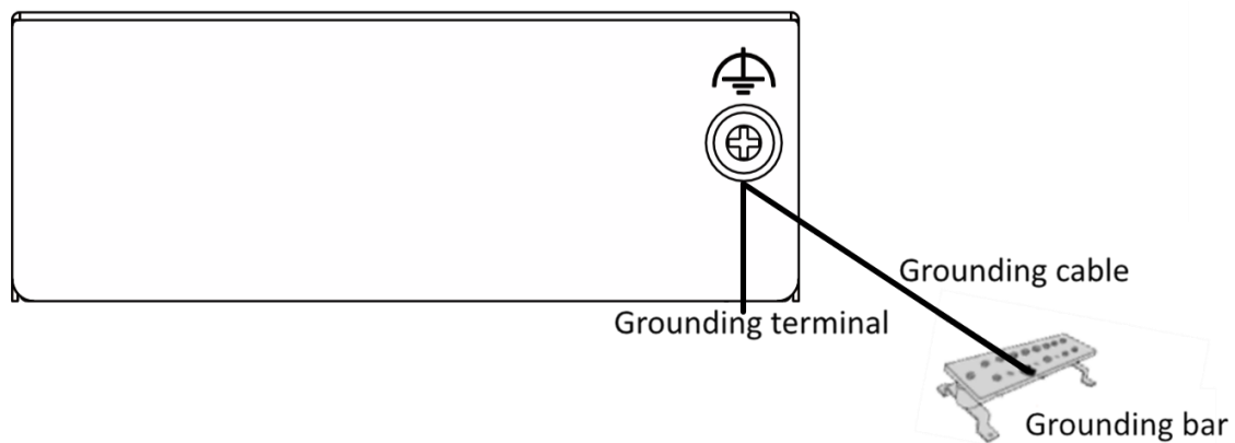
Figure 3-1 Grounding with Grounding Bar
