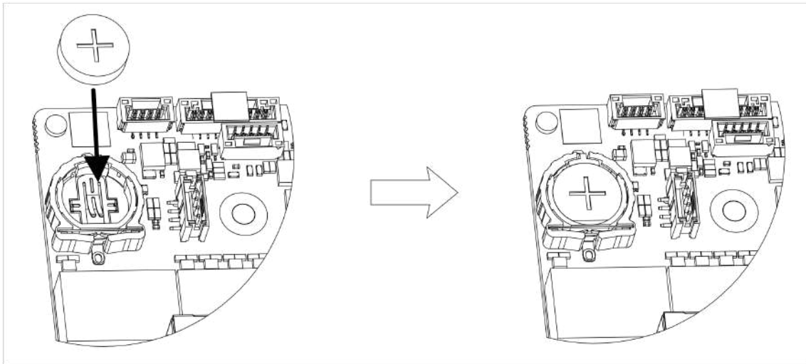
Figure 1-12 Replace Battery
