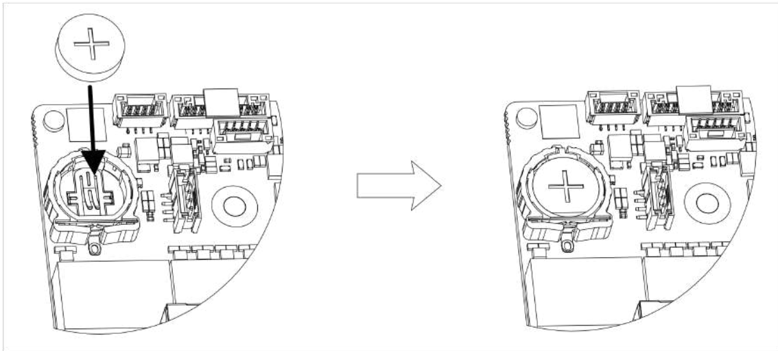
Figure 1-12 Replace Battery
