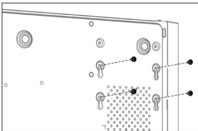
Figure 1-10 Fix HDD to Device Bottom
