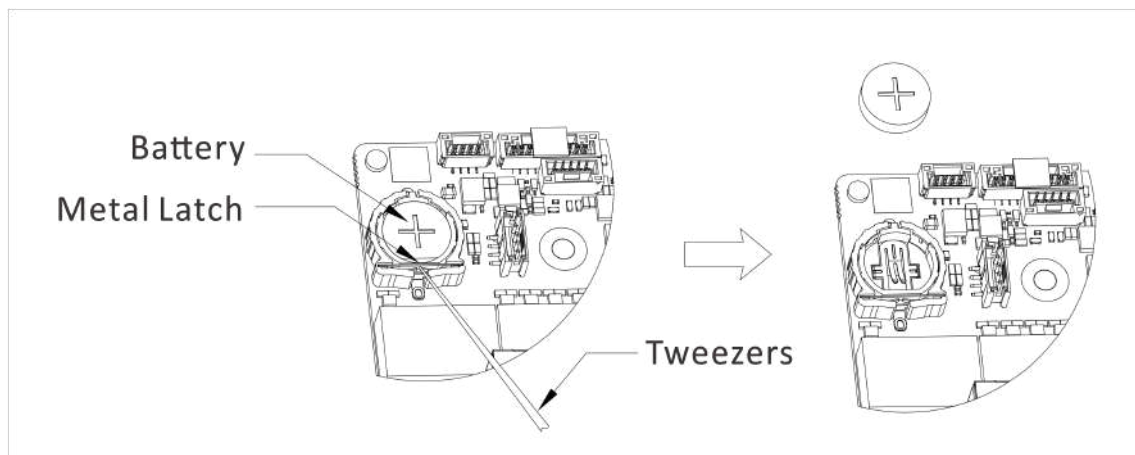
Figure 1-11 Remove Battery
