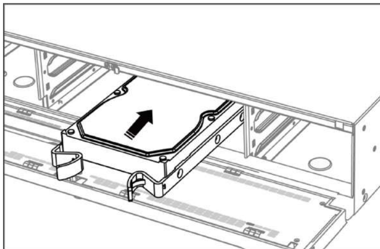
Figure 1-7 Insert HDD
