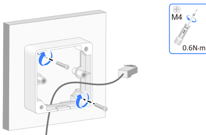
Figure 1-8 Feed Cable
