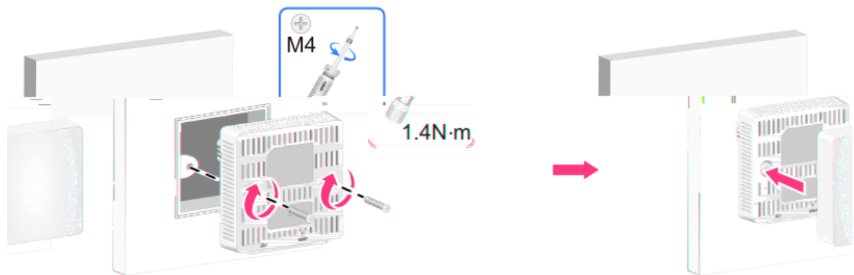
Figure 1-4 Secure Device to Junction Box
