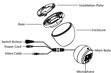
Figure 1-5 Overview of Type V Camera
