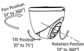
Figure 2-9 3-Axis Adjustment
