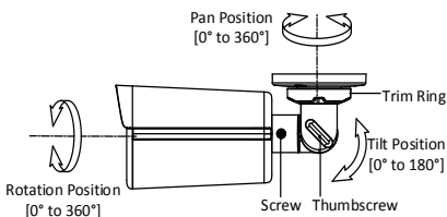
Figure 2-2 3-Axis Adjustment
