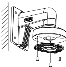
Figure 2-13 Fix the Installation Plate
