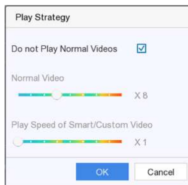
Figure 3-6 Play Strategy
