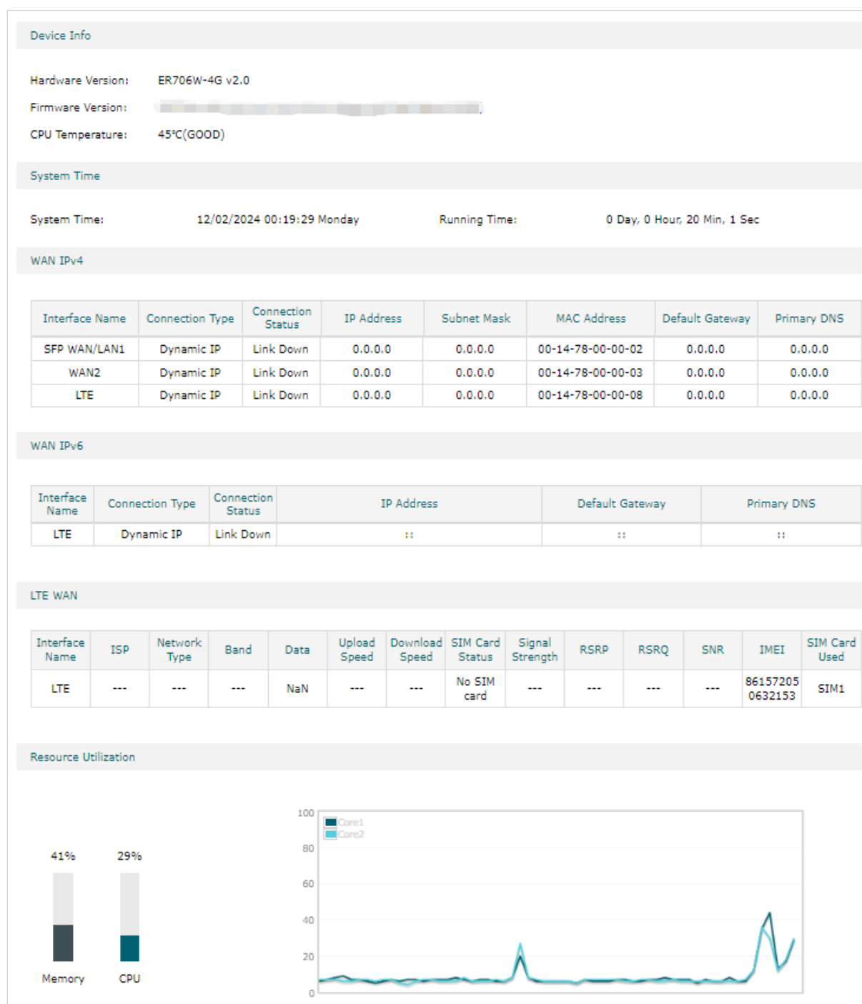
Figure 1-1 System Status
