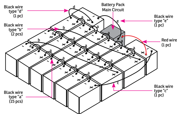
Battery connection diagram
