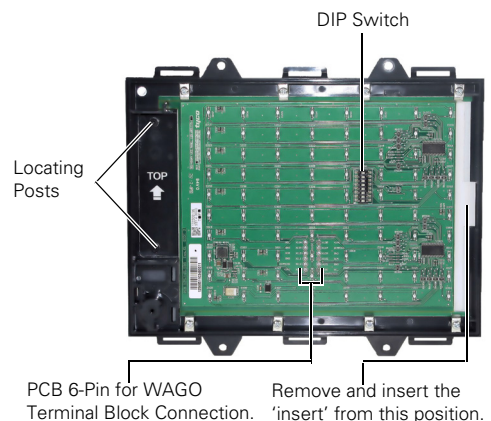
Fig. 9: Zonal Display - Rear View of Front Display
