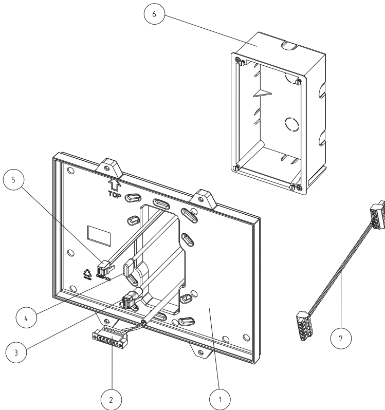
Fig. 1: Installation Overview of Shallow Back Cover Mounting Kit - To be mounted with compact network repeater
