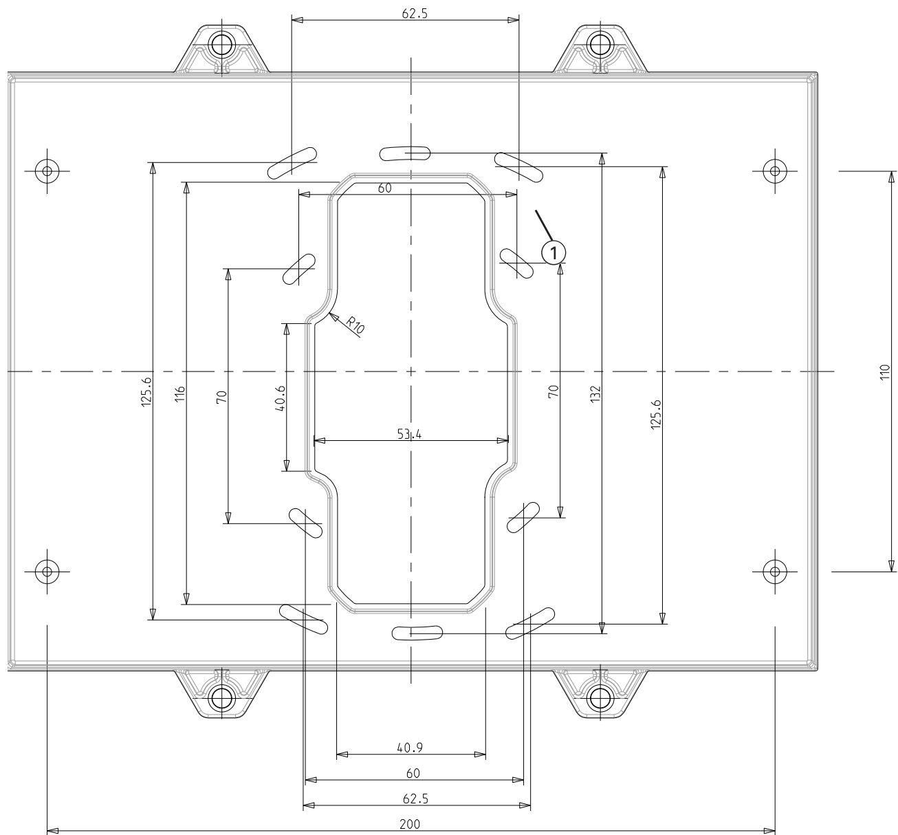
Fig. 8: FC1DS Fully Functional Repeater Shallow/FC1D2 FireClass FC700 series Display Only Repeater -Overall and Fixing Dimensions 1 – Slots
