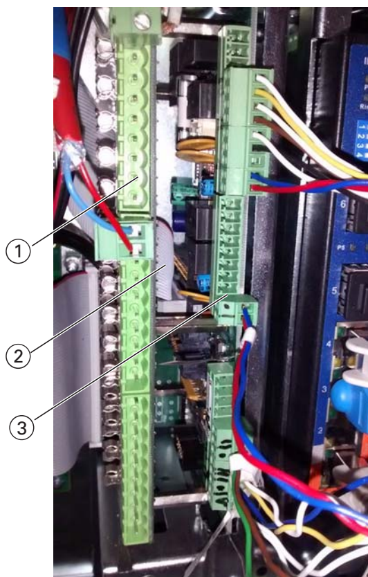
Fig. 21: IOB800 Positioning 1–Hosted board (FB800 in this case) 2–Ribbon cable 3–IOB800
